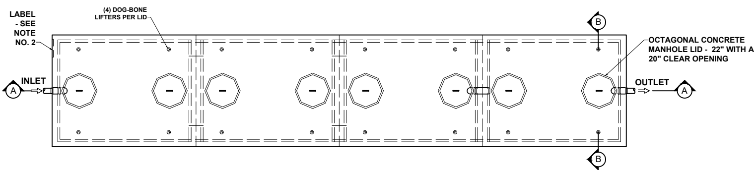
PLAN VIEW
